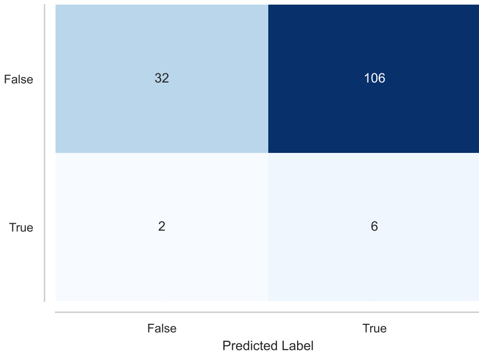
Confusion Matrix - LR
